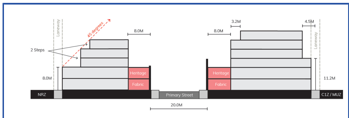
Figure 1: Indicative Cross Section and Measurements
