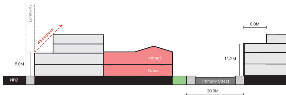
Figure 1: Indicative cross section and measurements
