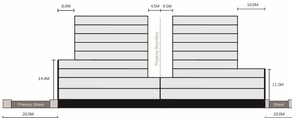
Figure 2: Indicative cross sections and measurements
